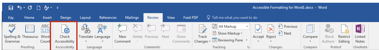
FIGURE 10 ACCESSIBILITY CHECKER
